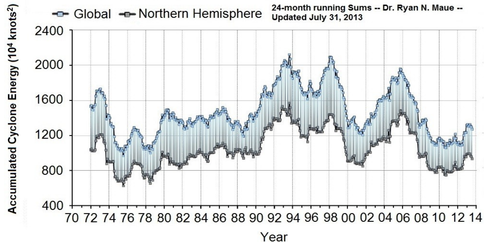
Global Tropical Cyclone Accumulated Cyclone Energy (ACE)
